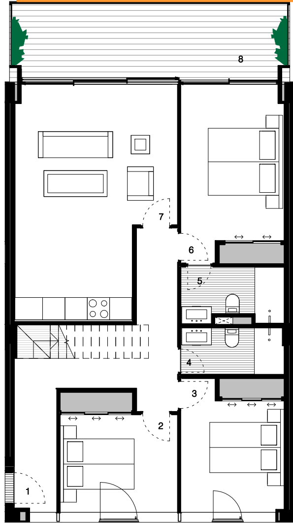
APARTMENT LAYOUT 1 : 100
