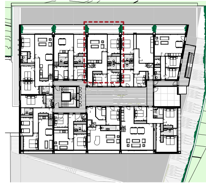
APARTMENT LOCATION. SIXTH FLOOR 1 : 500
