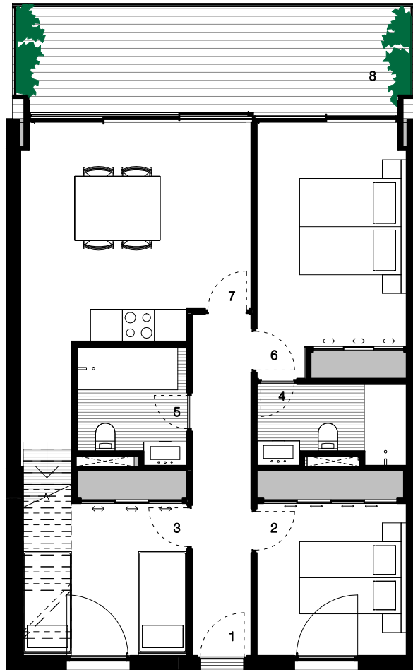
APARTMENT LAYOUT 1 : 100
