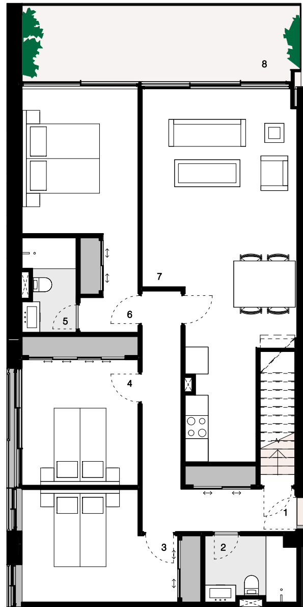
APARTMENT LAYOUT 1 : 100
