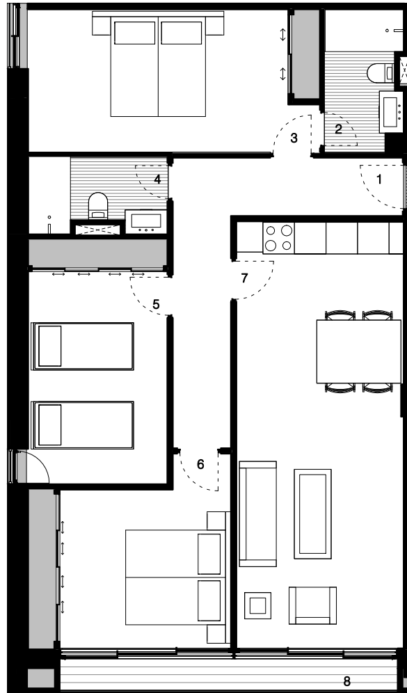
APARTMENT LAYOUT 1 : 100
