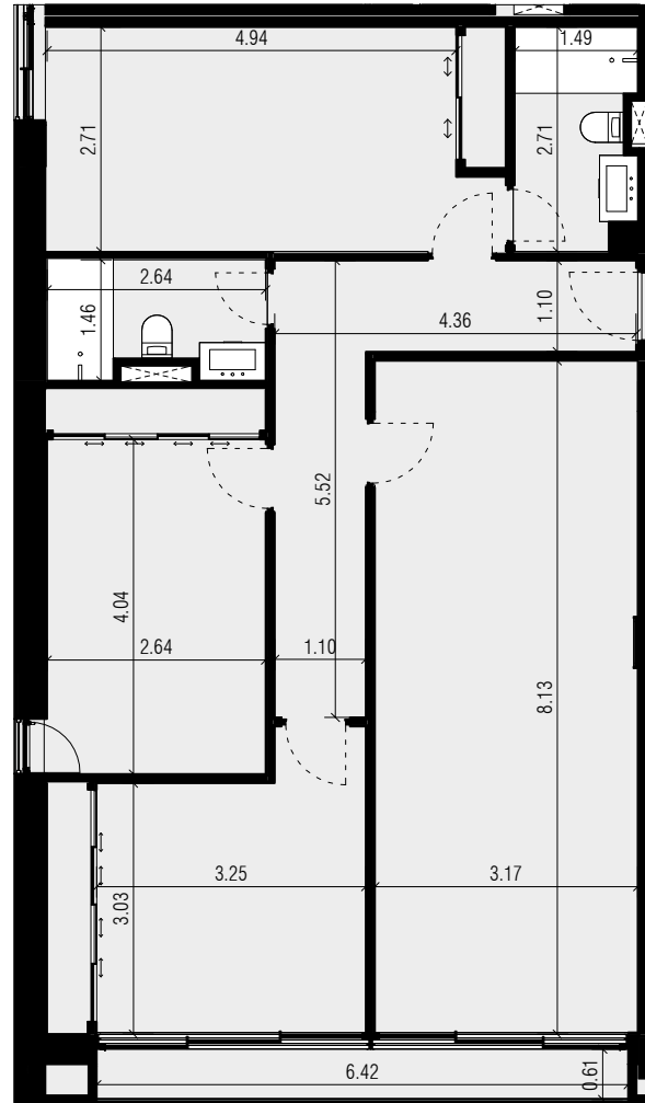
AREA AND DIMENSIONS 1 : 100
