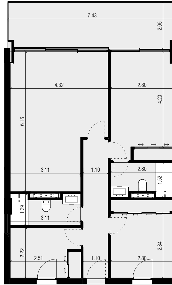
AREA AND DIMENSIONS 1 : 100
