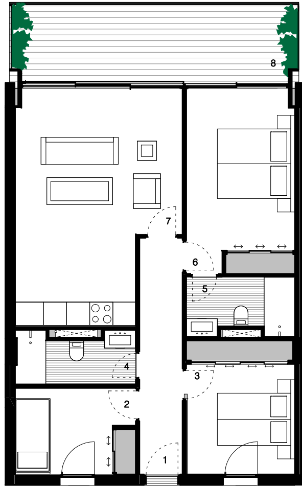
APARTMENT LAYOUT 1 : 100
