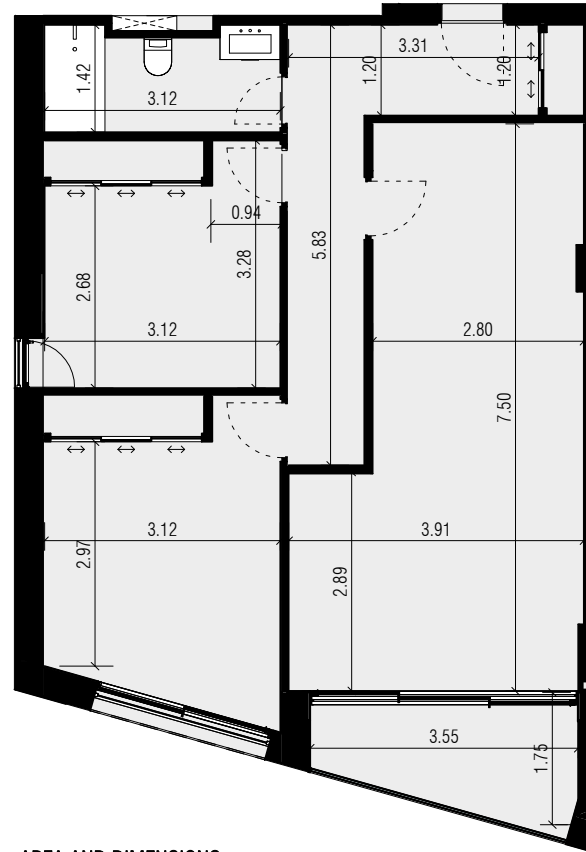
AREA AND DIMENSIONS 1 : 100
