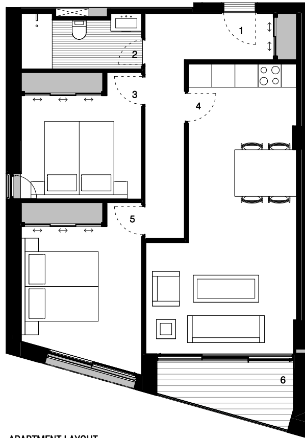
APARTMENT LAYOUT 1 : 100
